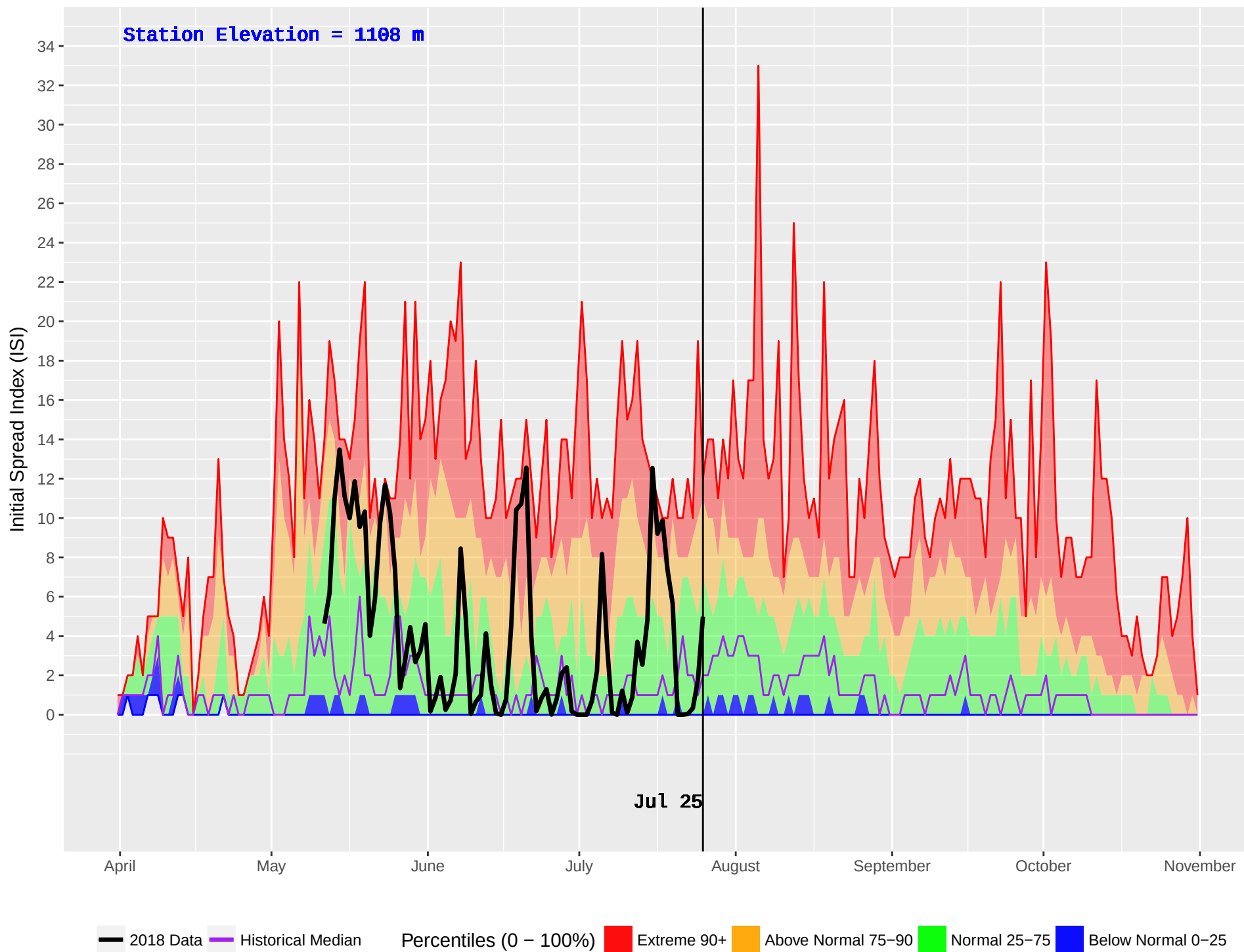
MATHEW (263) : Historical (1987–2016) and Current (2018) Noon Initial Spread Index (ISI)
