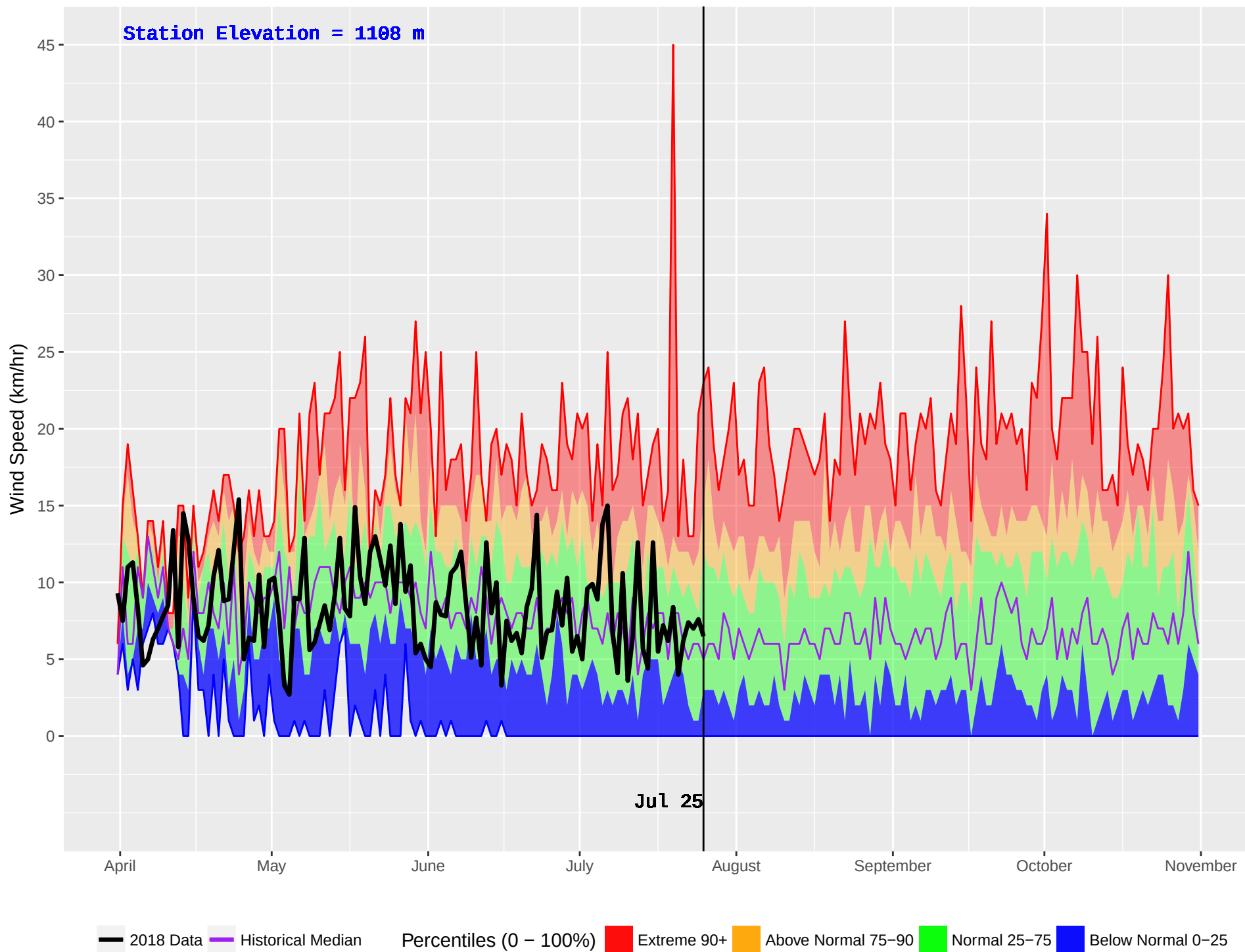
MATHEW (263) : Historical (1987–2016) and Current (2018) Noon Wind Speed
