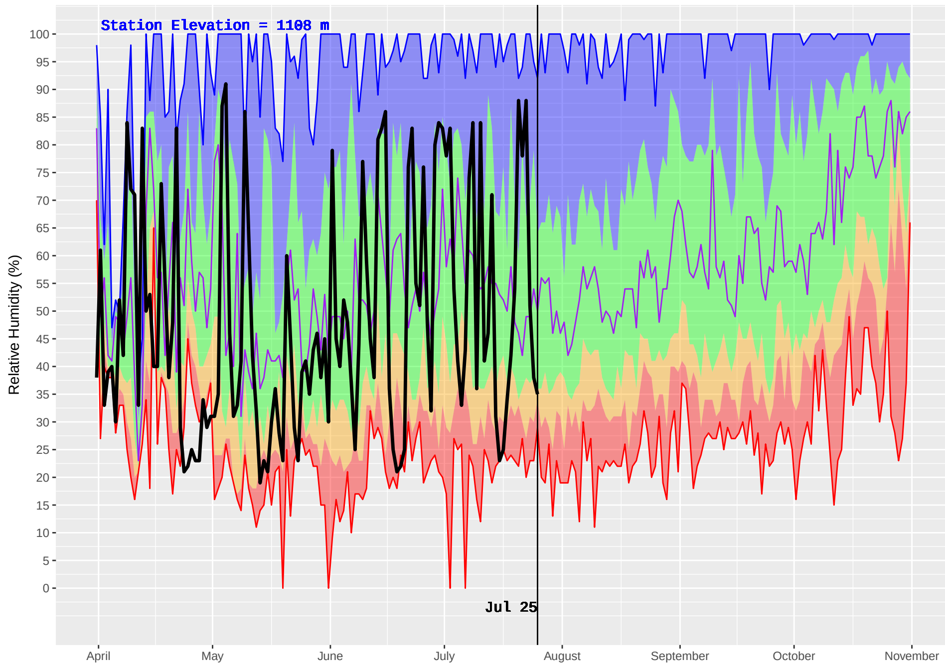
MATHEW (263) : Historical (1987–2016) and Current (2018) Noon Relative Humidity
