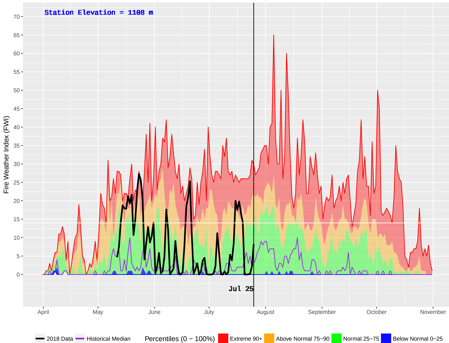
MATHEW (263) : Historical (1987–2016) and Current (2018) Noon Fire Weather Index (FWI)
