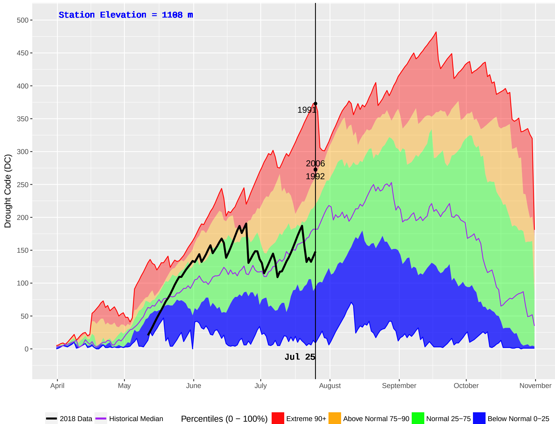
MATHEW (263) : Historical (1987–2016) and Current (2018) Noon Drought Code (DC)
