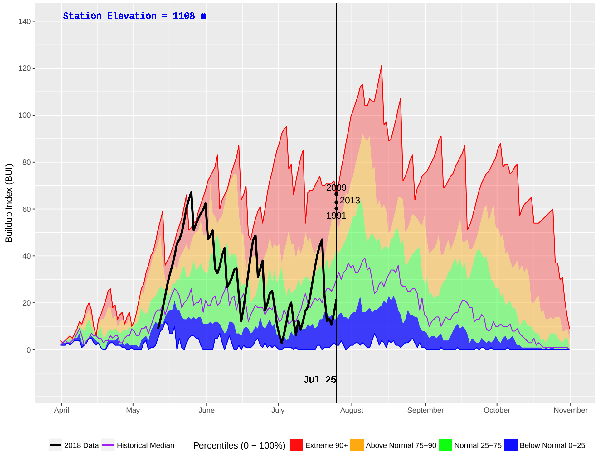
MATHEW (263) : Historical (1987–2016) and Current (2018) Noon Buildup Index (BUI)
