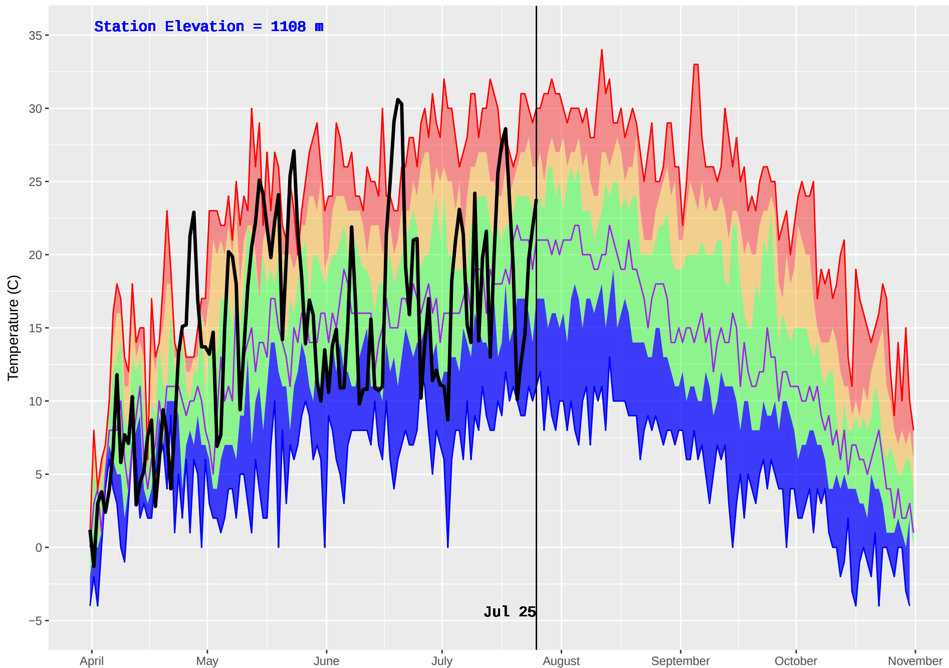
MATHEW (263) : Historical (1987–2016) and Current (2018) Noon Temperature
